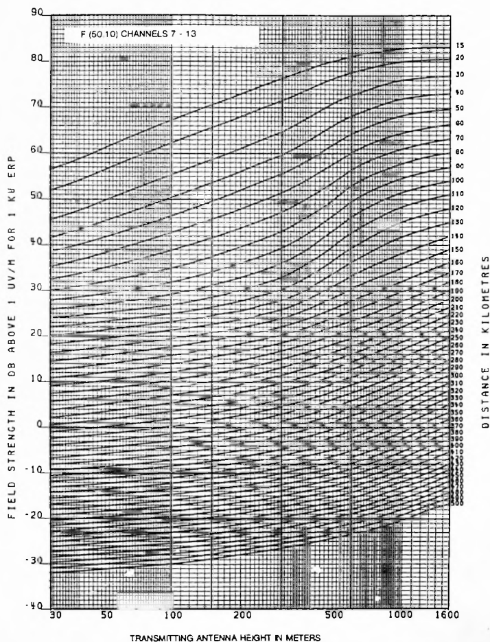
FCC 73.699 Figure 10a
