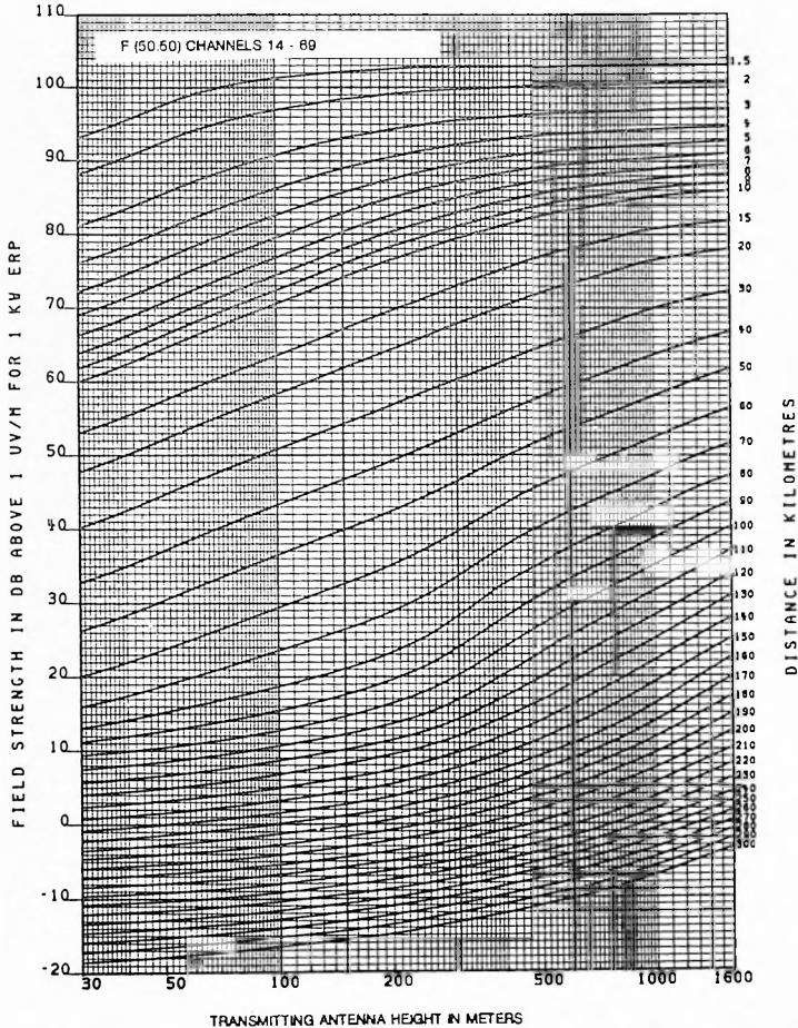
FCC 73.699 Figure 10b
