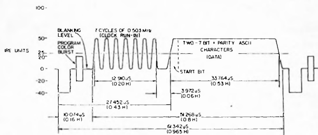
FIGURE 17 A. LINE 21 FIELD 1 DATA SIGNAL FORMAT
