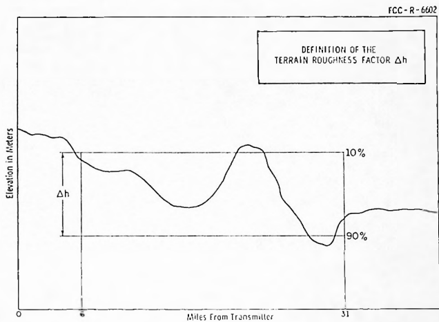
FCC § 73.333 FIGURE 4 (new)
