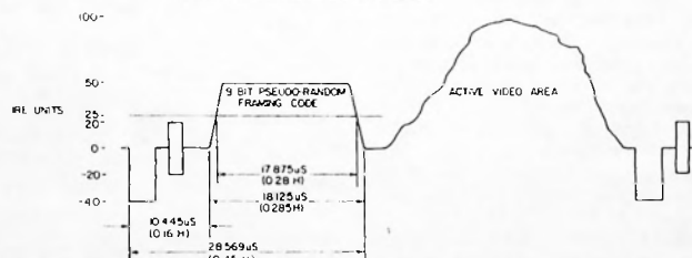
FIGURE 17 C. LINE 21 FIELD TWO FRAMING CODE
