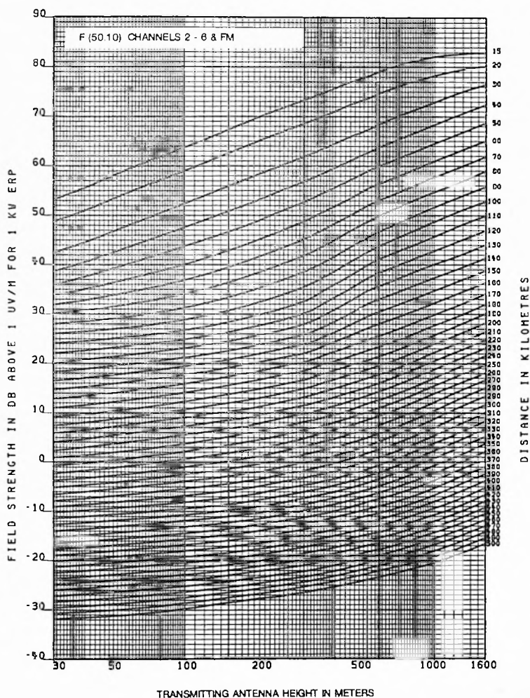
FCC 73.699 Figure 9a
