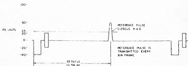
FIGURE 17 B. ADAPTIVE EQUALIZER REFERENCE PULSE
