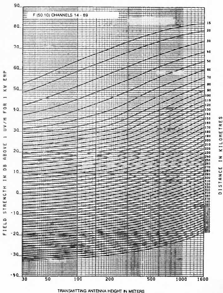
FCC 73.699 Figure 10c
