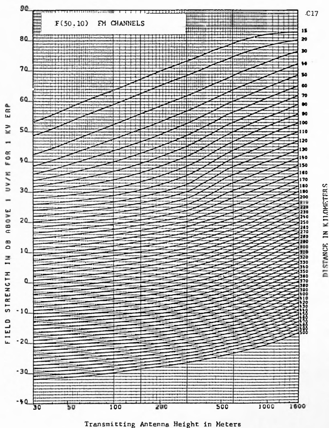
FCC 873.333 FIGURE 1a
